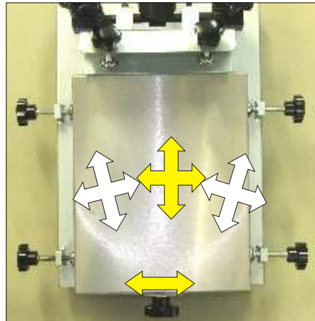
Micro adjustments. Print Bed can move back and forth as well as sideways and angled.
